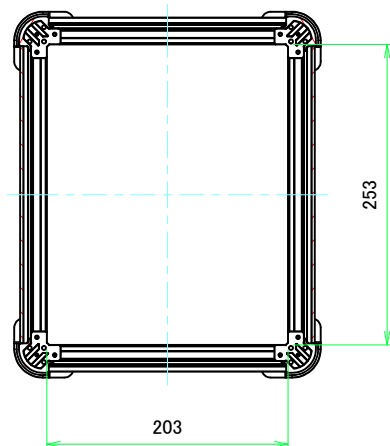
B-B (1:4.5)
