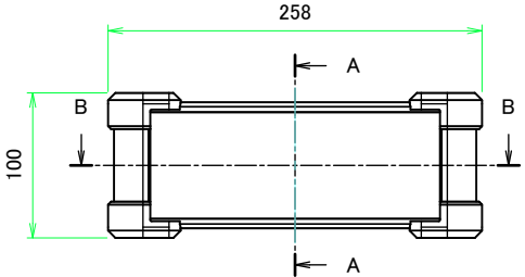
A view
