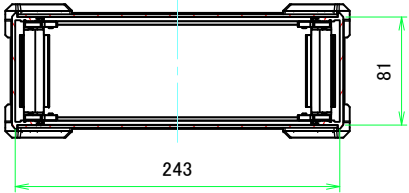
C-C (1:4)
