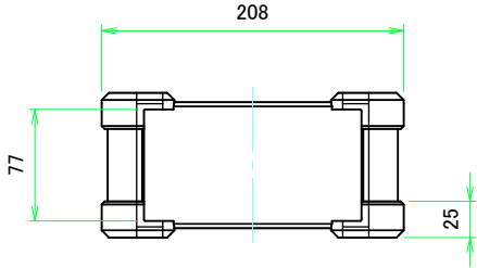
C view
