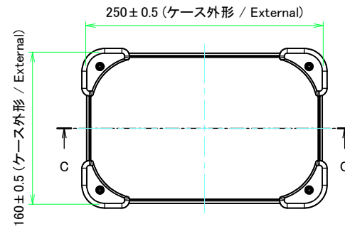
E view
