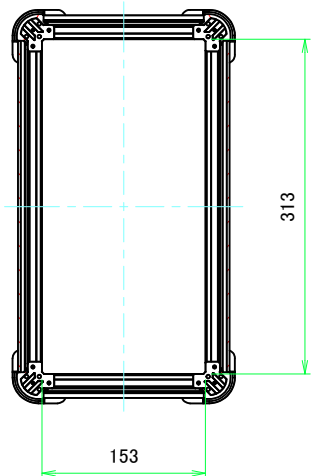
B-B (1:5)
