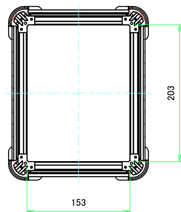
B-B (1:4)
