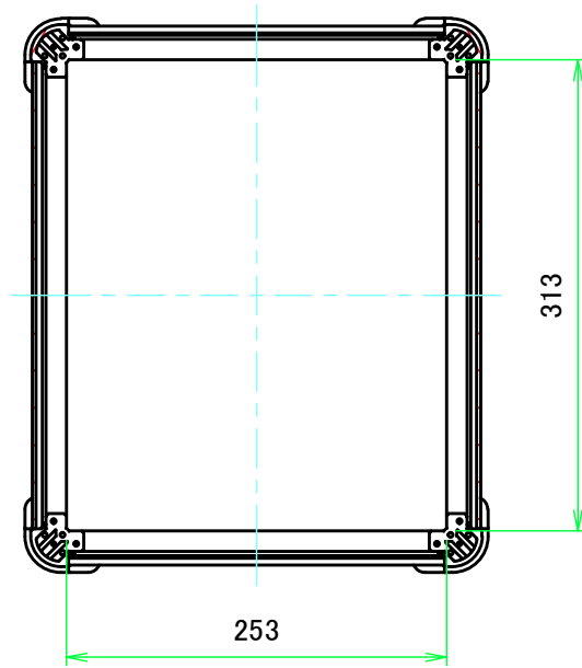
B-B ( 1:5.5 )
