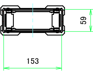
C-C (1:6)
