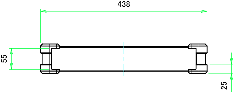
C view
