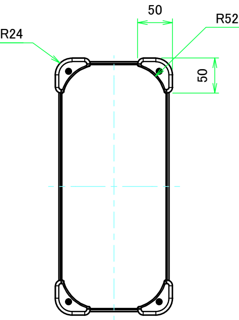
F view
