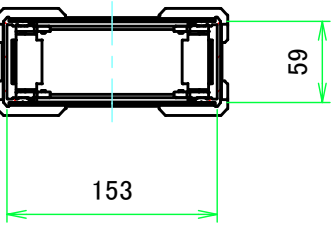
C-C (1:5.5)
