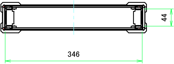
A-A (1:5.5)
