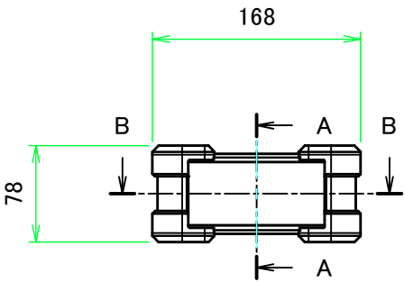
A view
