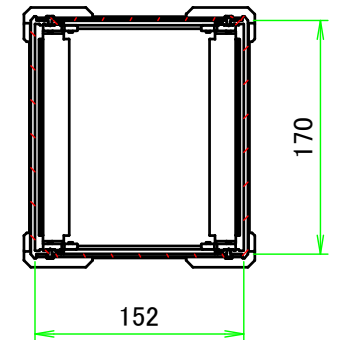
C-C ( 1 :5.5 )
