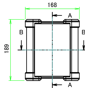
A view
