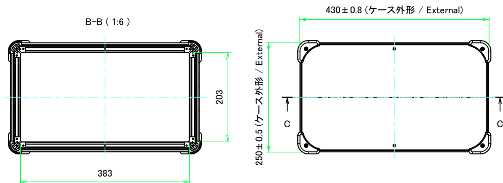
E view
