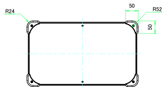
F view
