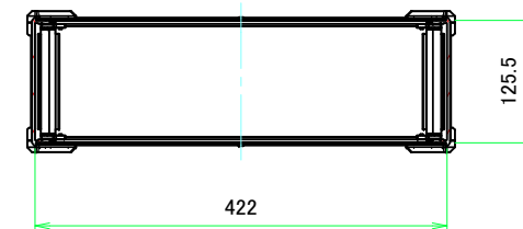
C-C (1:6)
