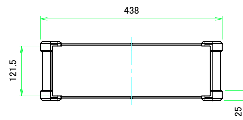
C view
