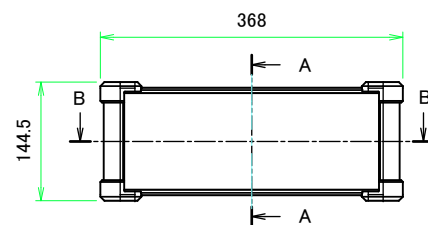
A view
