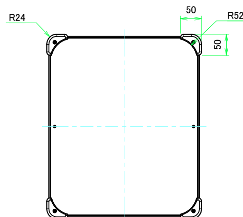
F view
