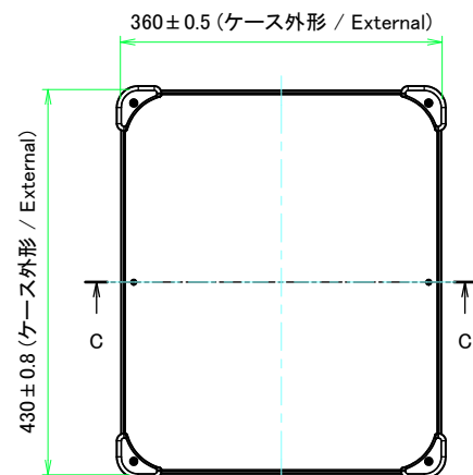
E view
