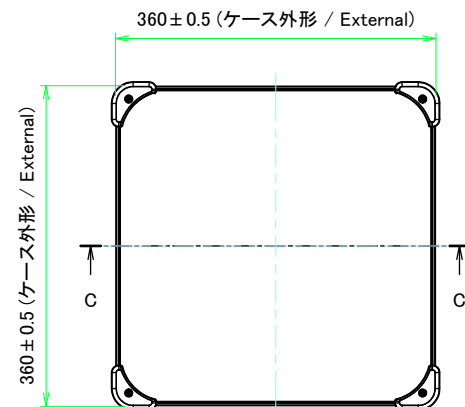
E view
