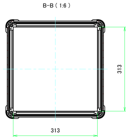
D view
