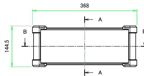
A view
