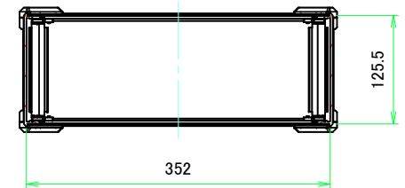
C-C (1:5.5)
