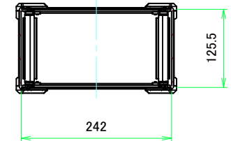
C-C (1:6)
