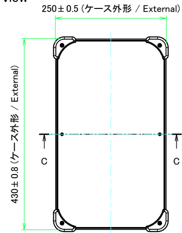
E view
