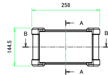
A view
