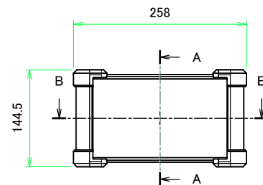
A view
