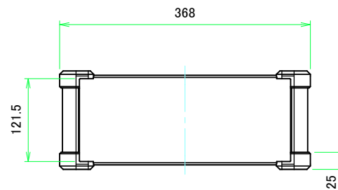
C view
