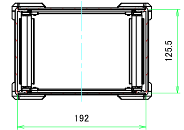
C-C (1:4)
