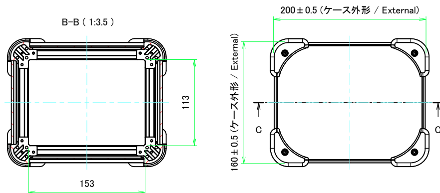
E view
