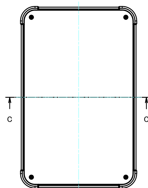
E view
