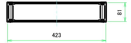
C-C (1:7)
