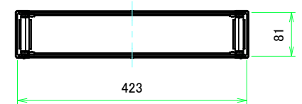
C-C (1:7)
