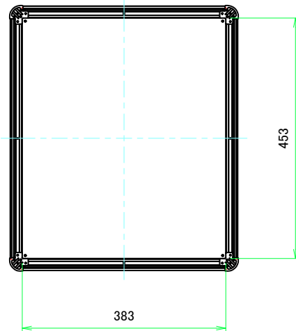
B-B (1:7)
