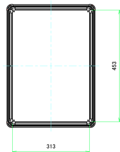
B-B (1:6.5)
