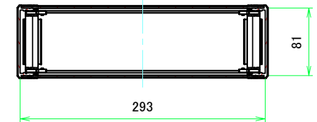
C-C (1:4.5)
