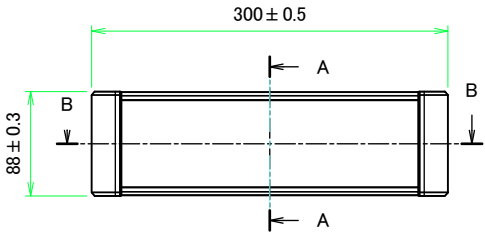
A view
