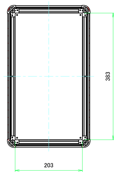
B-B (1:5)
