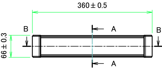
A view
