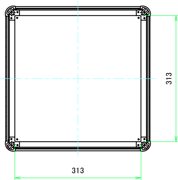
B-B ( 1:5.5 )
