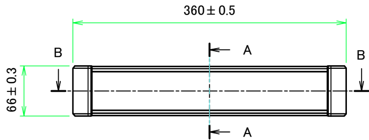
A view
