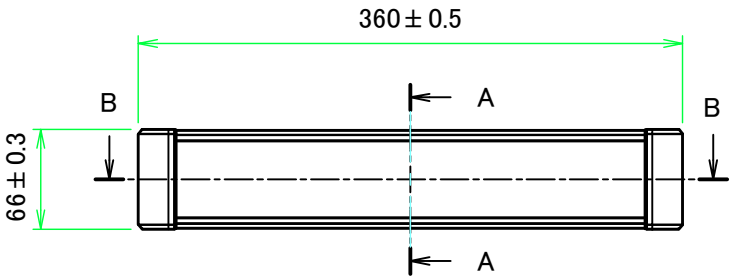
A view
