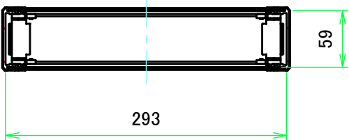
C-C ( 1:5.5 )
