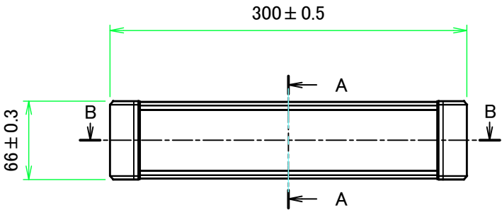
A view
