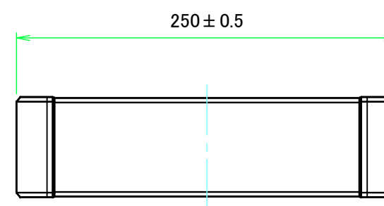
C view
