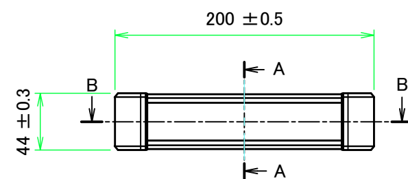
A view
