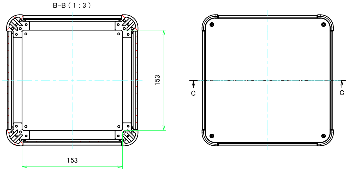
E view
