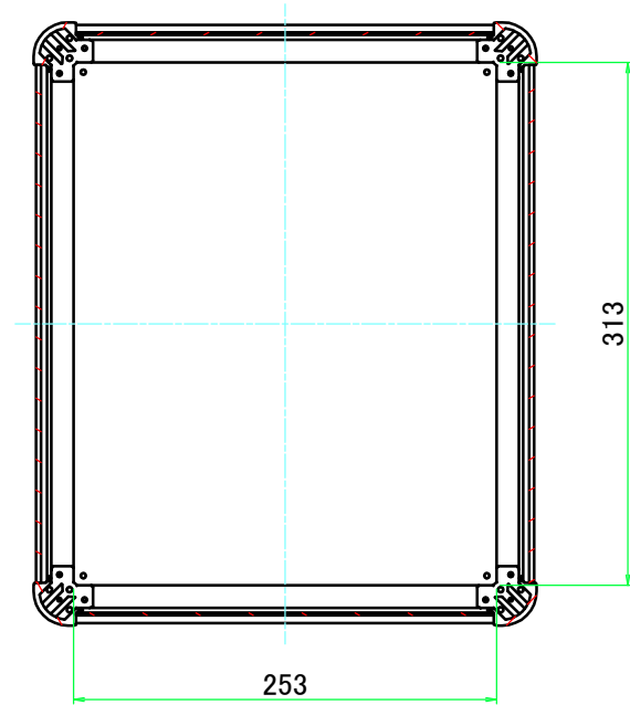
B-B (1:5)
