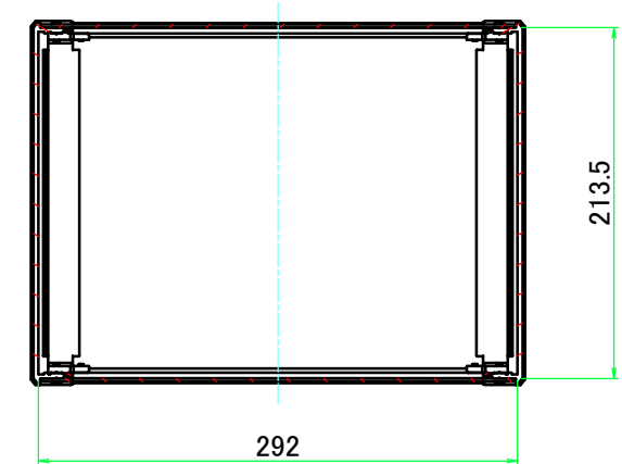
C-C (1:5)
