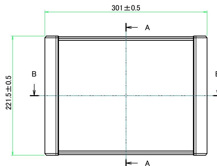
A view
