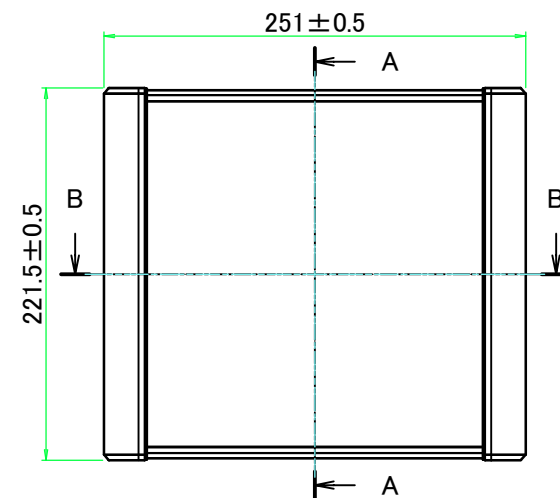
A view
