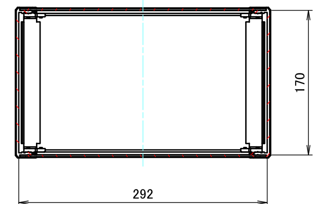
C-C ( 1 :4.5 )
