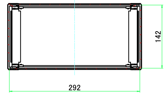
C-C (1:5)
