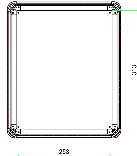
B-B (1:5)
