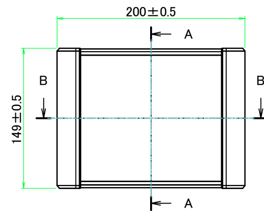
A view
