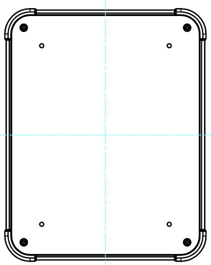
F view
