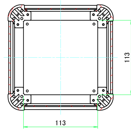
B-B (1:3)
