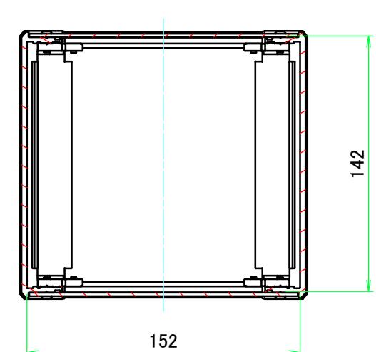
C-C (1:3)
