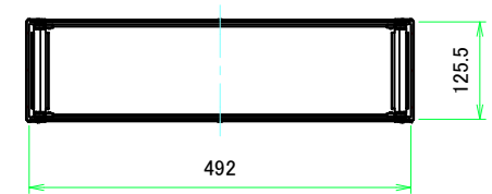
C-C (1:7.5)
