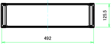
C-C (1:7)
