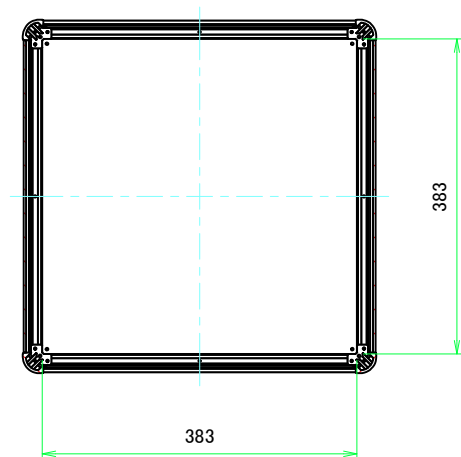
B-B (1:6.5)
