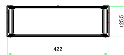
C-C (1:6.5)
