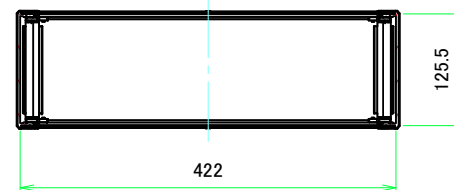
C-C (1:6)
