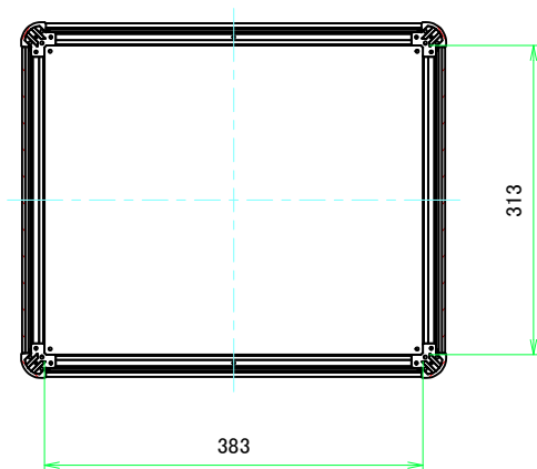
B-B (1:6)
