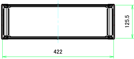
C-C (1:6)
