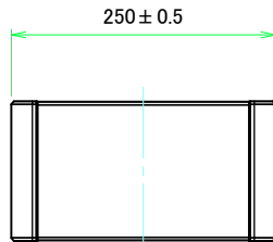
C view
