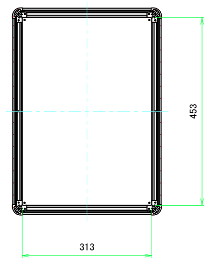
B-B (1:6.5)
