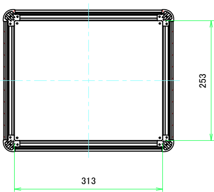
D view
