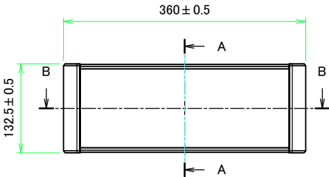
A view
