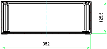
C-C (1:5)
