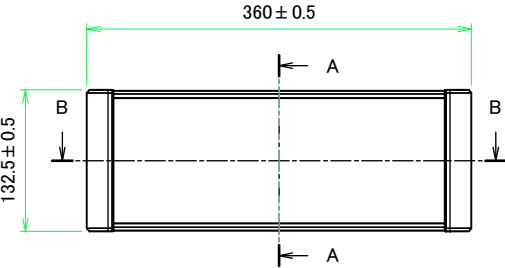
F view
